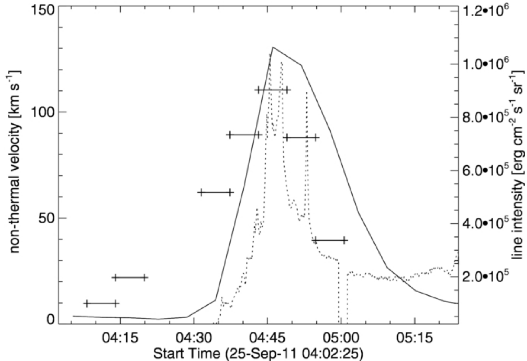
Figure 9. from The Relationship between Extreme Ultraviolet Non-thermal Line Broadening and High-energy Particles during Solar Flares Kawate & Imada 2013 ApJ 775 122 doi:10.1088/0004-637X/775/2/122 https://dx.doi.org/10.1088/0004-637X/775/2/122 © 2013. The American Astronomical Society. All rights reserved.
