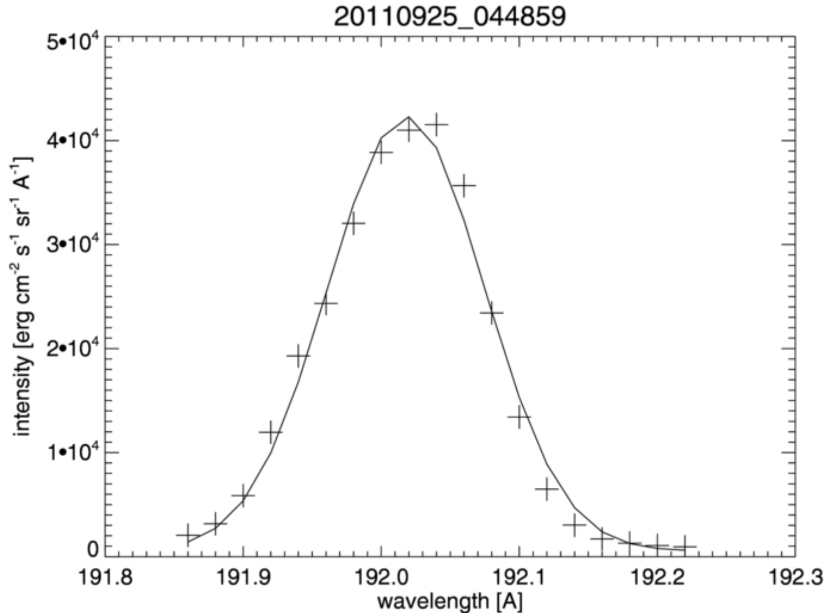
Figure 8. from The Relationship between Extreme Ultraviolet Non-thermal Line Broadening and High-energy Particles during Solar Flares Kawate & Imada 2013 ApJ 775 122 doi:10.1088/0004-637X/775/2/122 https://dx.doi.org/10.1088/0004-637X/775/2/122 © 2013. The American Astronomical Society. All rights reserved.
