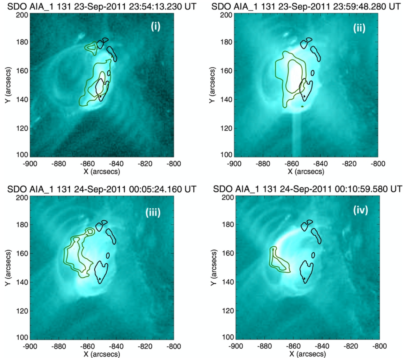
Figure 6. from The Relationship between Extreme Ultraviolet Non-thermal Line Broadening and High-energy Particles during Solar Flares Kawate & Imada 2013 ApJ 775 122 doi:10.1088/0004-637X/775/2/122 https://dx.doi.org/10.1088/0004-637X/775/2/122
