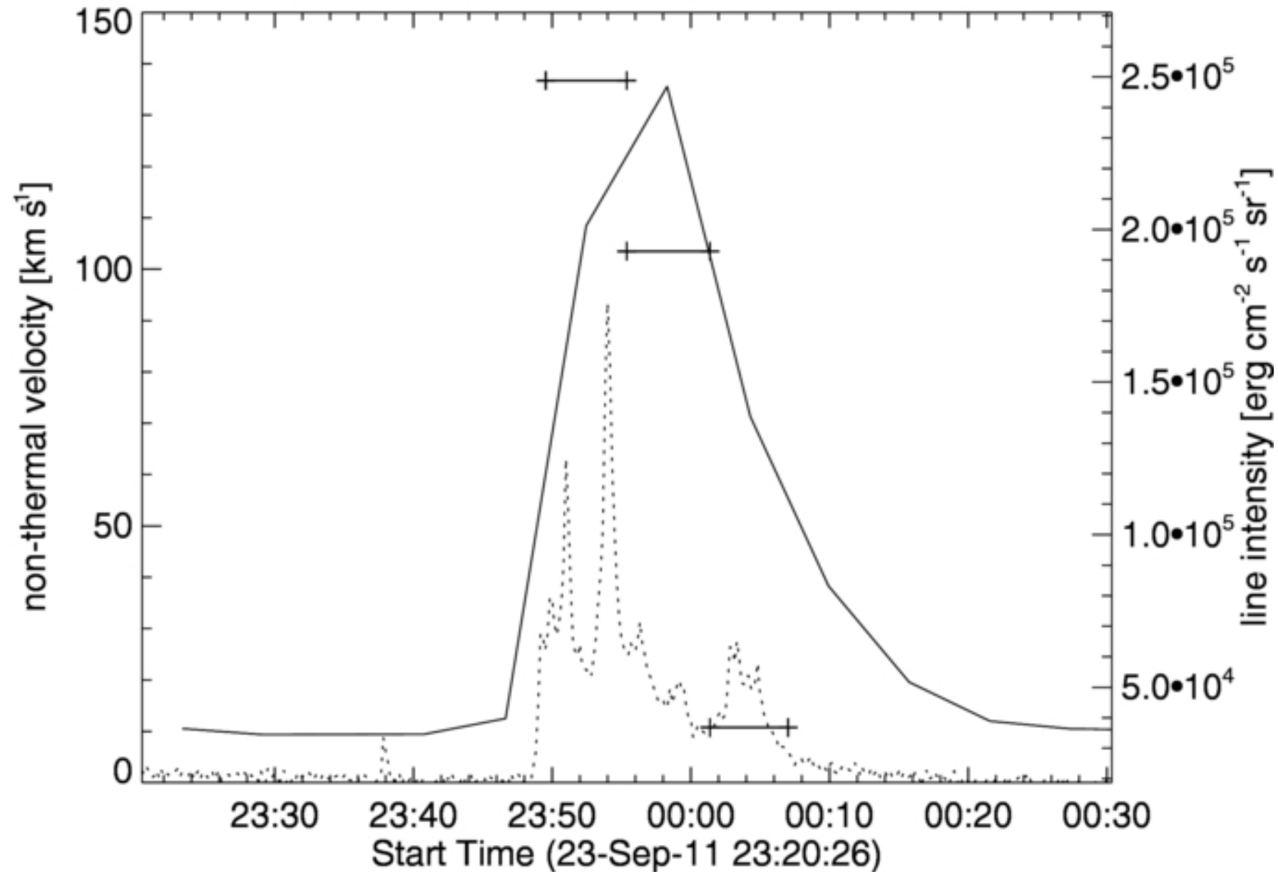
Figure 4. from The Relationship between Extreme Ultraviolet Non-thermal Line Broadening and High-energy Particles during Solar Flares Kawate & Imada 2013 ApJ 775 122 doi:10.1088/0004-637X/775/2/122 https://dx.doi.org/10.1088/0004-637X/775/2/122 © 2013. The American Astronomical Society. All rights reserved.
