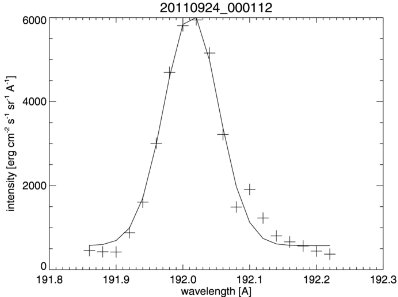
Figure 3. from The Relationship between Extreme Ultraviolet Non-thermal Line Broadening and High-energy Particles during Solar Flares Kawate & Imada 2013 ApJ 775 122 doi:10.1088/0004-637X/775/2/122 https://dx.doi.org/10.1088/0004-637X/775/2/122 © 2013. The American Astronomical Society. All rights reserved.
