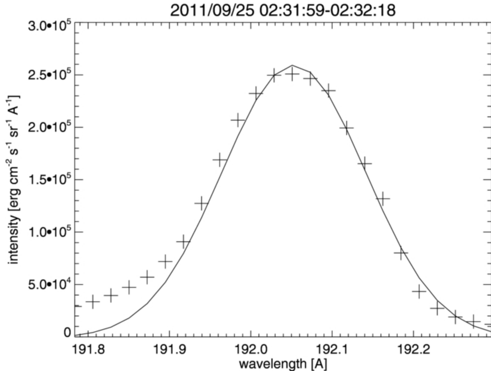
Figure 13. from The Relationship between Extreme Ultraviolet Non-thermal Line Broadening and High-energy Particles during Solar Flares Kawate & Imada 2013 ApJ 775 122 doi:10.1088/0004-637X/775/2/122 https://dx.doi.org/10.1088/0004-637X/775/2/122 © 2013. The American Astronomical Society. All rights reserved.
