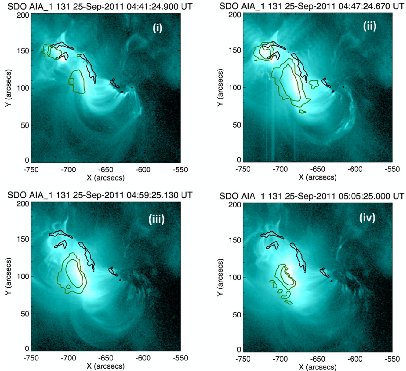
Figure 11. from The Relationship between Extreme Ultraviolet Non-thermal Line Broadening and High-energy Particles during Solar Flares Kawate & Imada 2013 ApJ 775 122 doi:10.1088/0004-637X/775/2/122 https://dx.doi.org/10.1088/0004-637X/775/2/122
