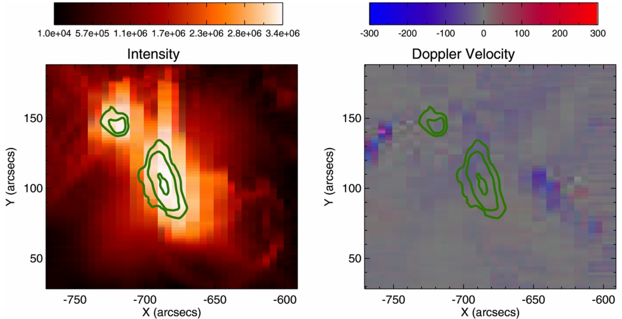
Figure 10. from The Relationship between Extreme Ultraviolet Non-thermal Line Broadening and High-energy Particles during Solar Flares Kawate & Imada 2013 ApJ 775 122 doi:10.1088/0004-637X/775/2/122 https://dx.doi.org/10.1088/0004-637X/775/2/122 © 2013. The American Astronomical Society. All rights reserved.
