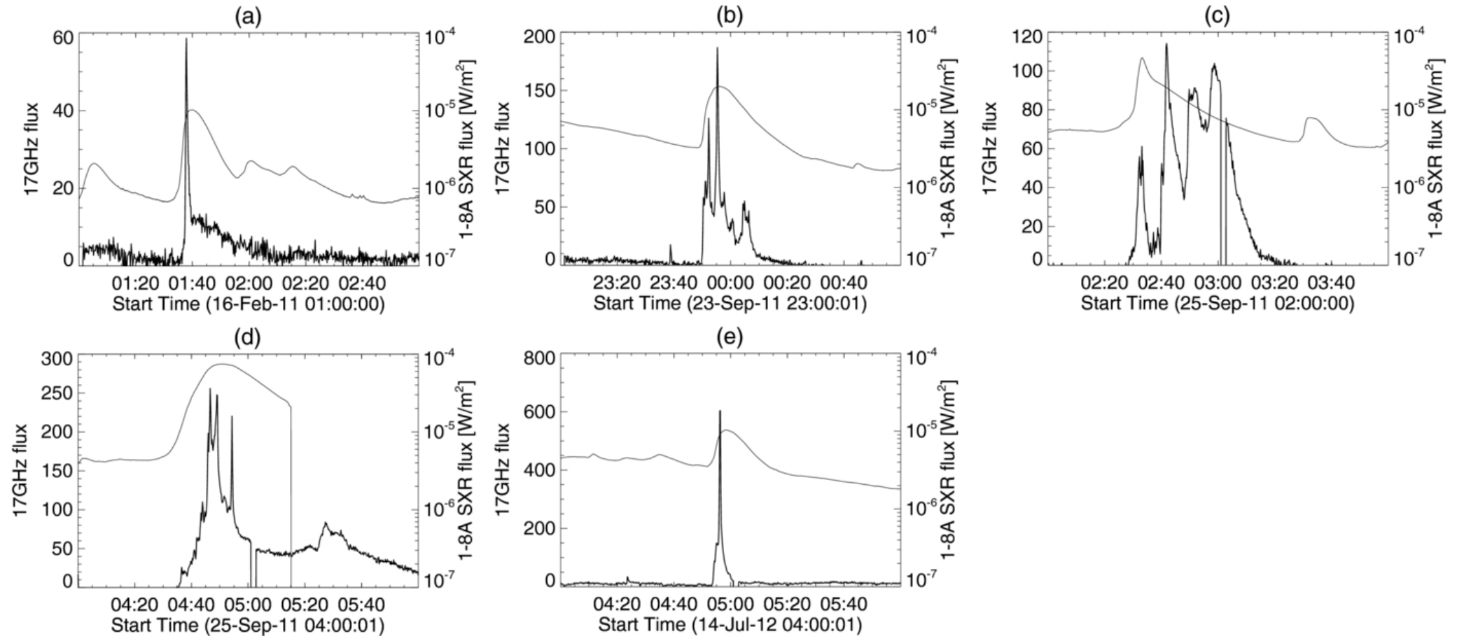
Figure 1. from The Relationship between Extreme Ultraviolet Non-thermal Line Broadening and High-energy Particles during Solar Flares Kawate & Imada 2013 ApJ 775 122 doi:10.1088/0004-637X/775/2/122 https://dx.doi.org/10.1088/0004-637X/775/2/122 © 2013. The American Astronomical Society. All rights reserved.
