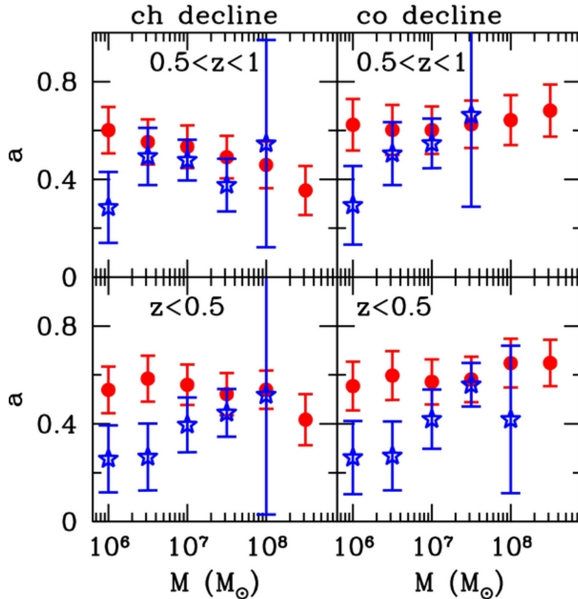
Figure 8. from The Evolution of Active Galactic Nuclei and their Spins Volonteri et al. 2013 ApJ 775 94 doi:10.1088/0004-637X/775/2/94 https://dx.doi.org/10.1088/0004-637X/775/2/94 © 2013. The American Astronomical Society. All rights reserved.
