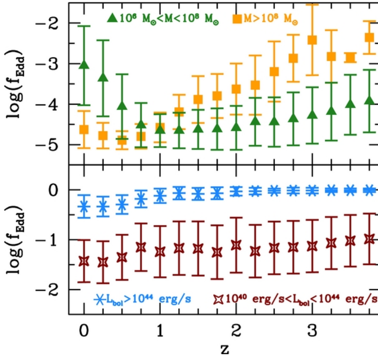
Figure 7. from The Evolution of Active Galactic Nuclei and their Spins Volonteri et al. 2013 ApJ 775 94 doi:10.1088/0004-637X/775/2/94 https://dx.doi.org/10.1088/0004-637X/775/2/94 © 2013. The American Astronomical Society. All rights reserved.
