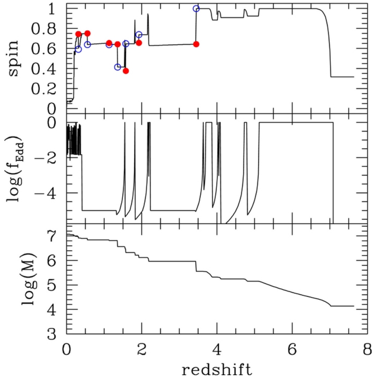
Figure 6. from The Evolution of Active Galactic Nuclei and their Spins Volonteri et al. 2013 ApJ 775 94 doi:10.1088/0004-637X/775/2/94 https://dx.doi.org/10.1088/0004-637X/775/2/94 © 2013. The American Astronomical Society. All rights reserved.
