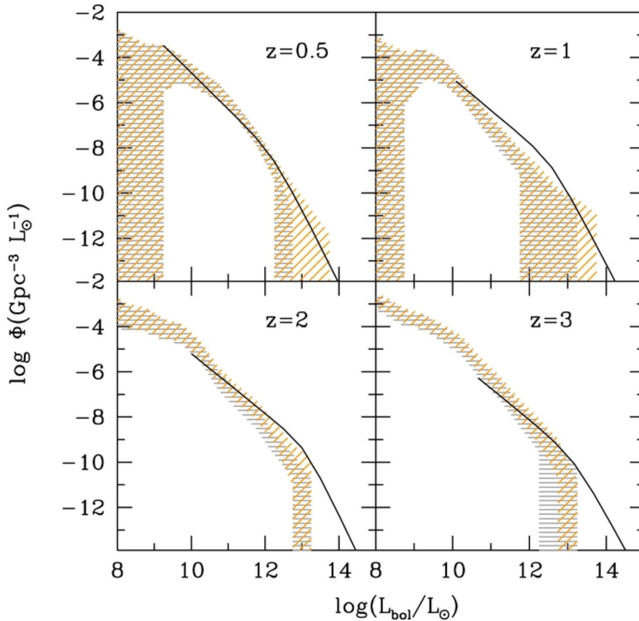
Figure 3. from The Evolution of Active Galactic Nuclei and their Spins Volonteri et al. 2013 ApJ 775 94 doi:10.1088/0004-637X/775/2/94 https://dx.doi.org/10.1088/0004-637X/775/2/94 © 2013. The American Astronomical Society. All rights reserved.
