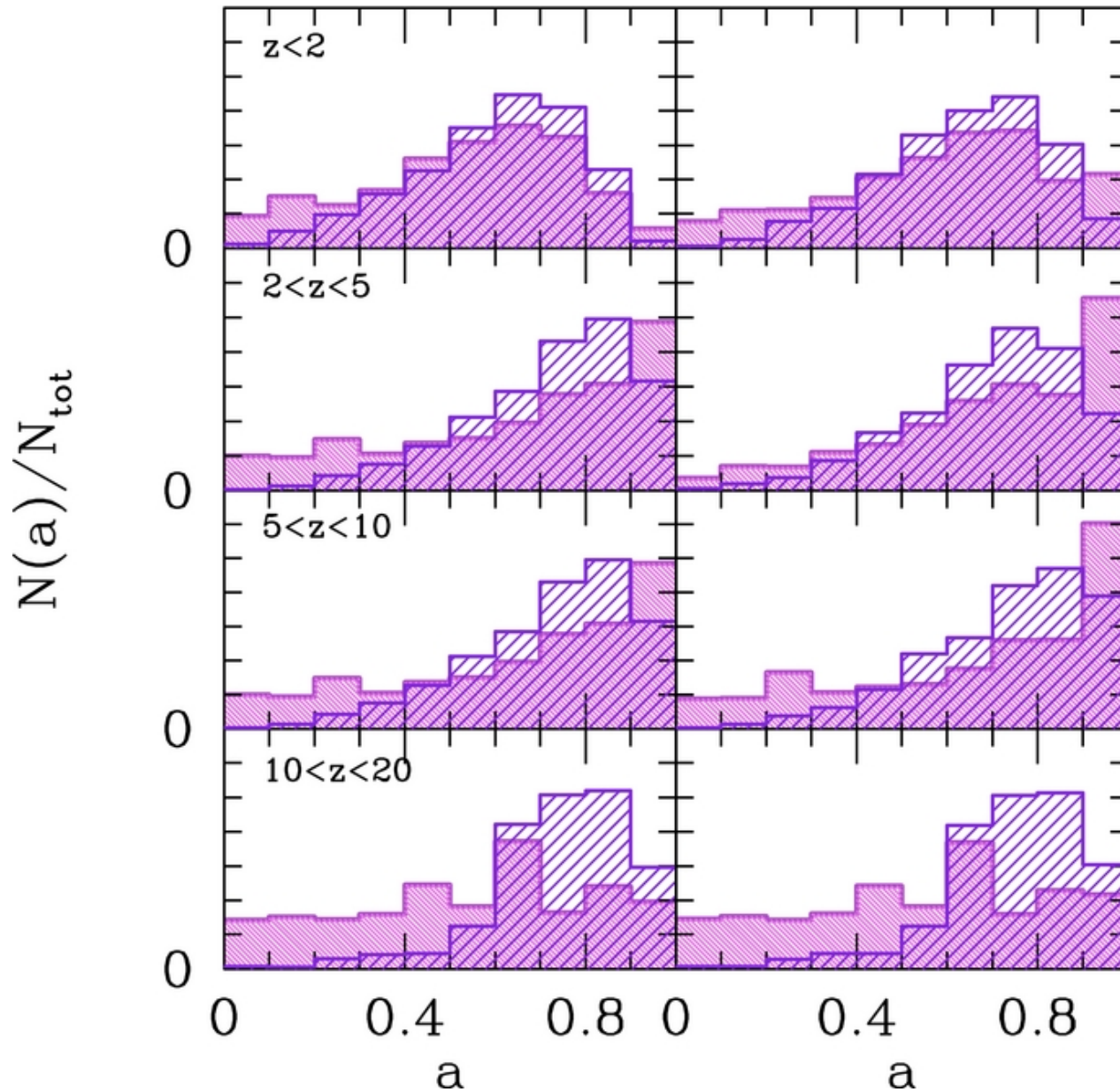
Figure 11. from The Evolution of Active Galactic Nuclei and their Spins Volonteri et al. 2013 ApJ 775 94 doi:10.1088/0004-637X/775/2/94 https://dx.doi.org/10.1088/0004-637X/775/2/94 © 2013. The American Astronomical Society. All rights reserved.
