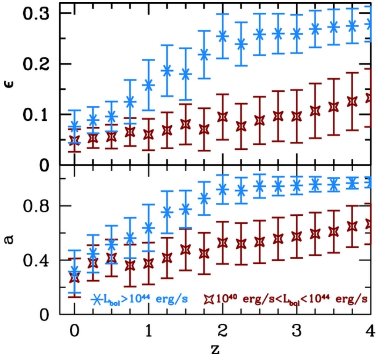
Figure 10. from The Evolution of Active Galactic Nuclei and their Spins Volonteri et al. 2013 ApJ 775 94 doi:10.1088/0004-637X/775/2/94 https://dx.doi.org/10.1088/0004-637X/775/2/94 © 2013. The American Astronomical Society. All rights reserved.
