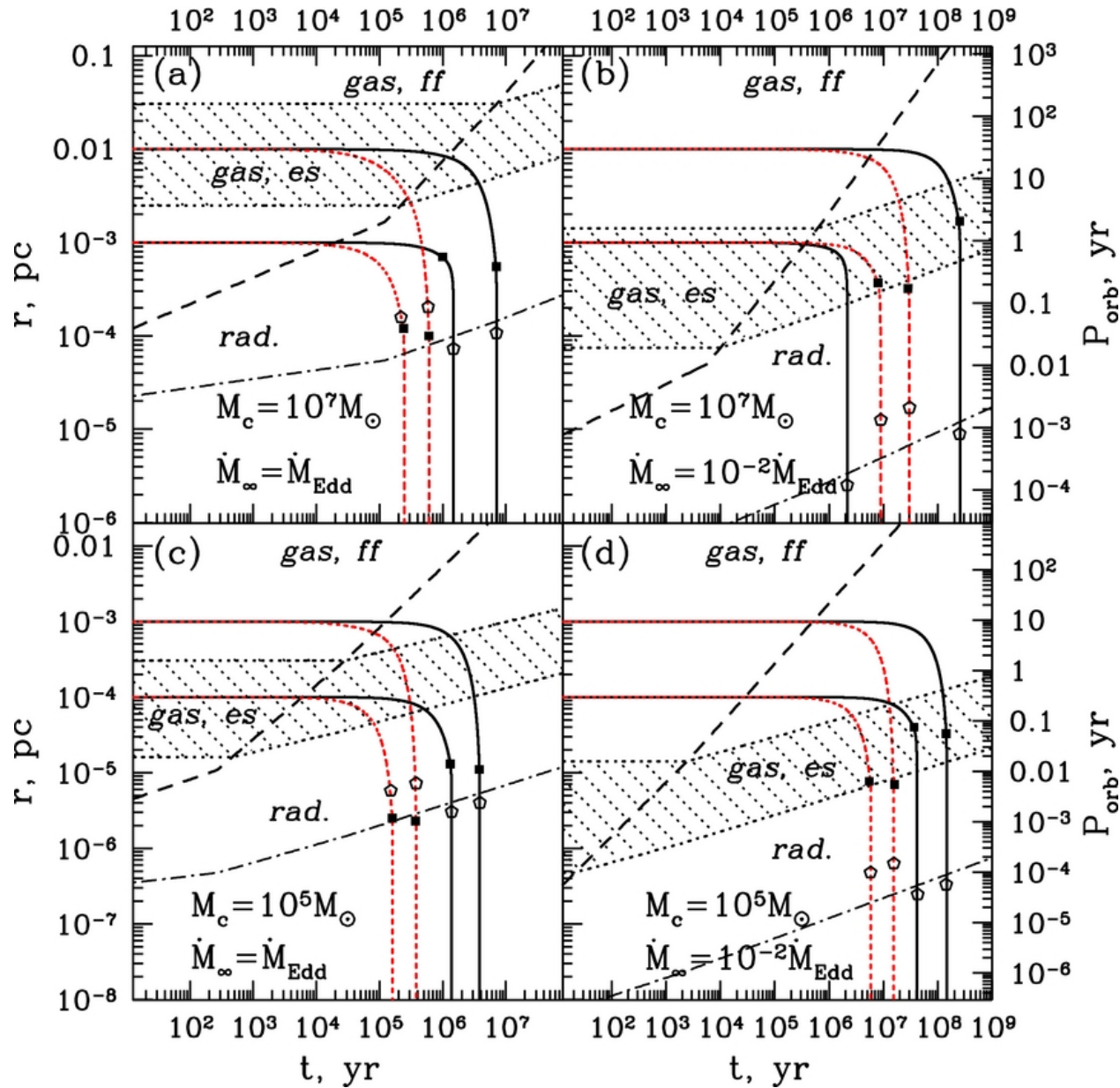
Figure 6. from Structure and Evolution of Circumbinary Disks around Supermassive Black Hole Binaries Rafikov 2013 ApJ 774 144 doi:10.1088/0004-637X/774/2/144 https://dx.doi.org/10.1088/0004-637X/774/2/144 © 2013. The American Astronomical Society. All rights reserved.
