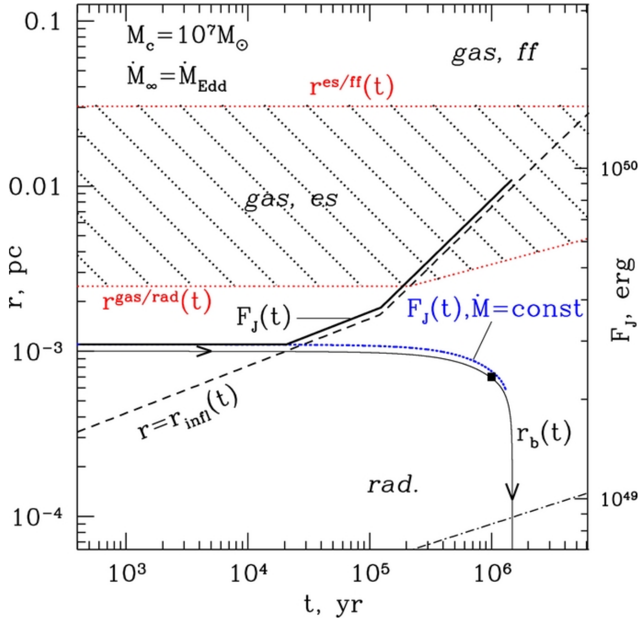
Figure 5. from Structure and Evolution of Circumbinary Disks around Supermassive Black Hole Binaries Rafikov 2013 ApJ 774 144 doi:10.1088/0004-637X/774/2/144 https://dx.doi.org/10.1088/0004-637X/774/2/144 © 2013. The American Astronomical Society. All rights reserved.
