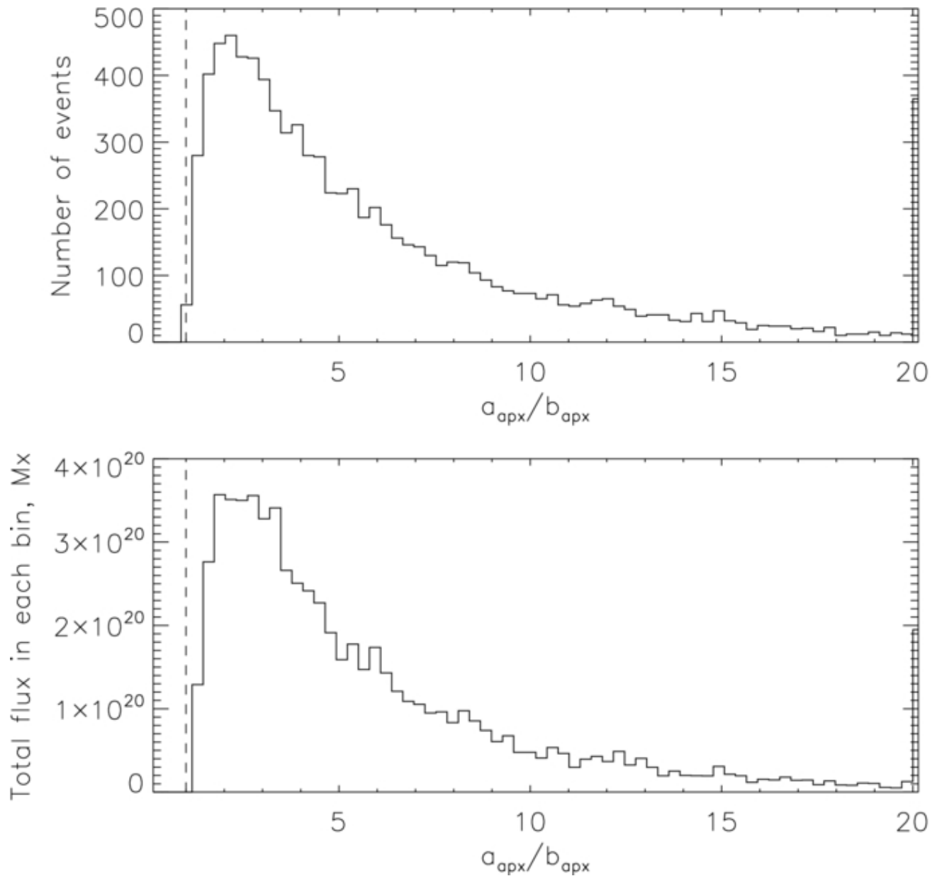
Figure 9. from On the Anisotropy in Expansion of Magnetic Flux Tubes in the Solar Corona Malanushenko & Schrijver 2013 ApJ 775 120 doi:10.1088/0004-637X/775/2/120 https://dx.doi.org/10.1088/0004-637X/775/2/120
