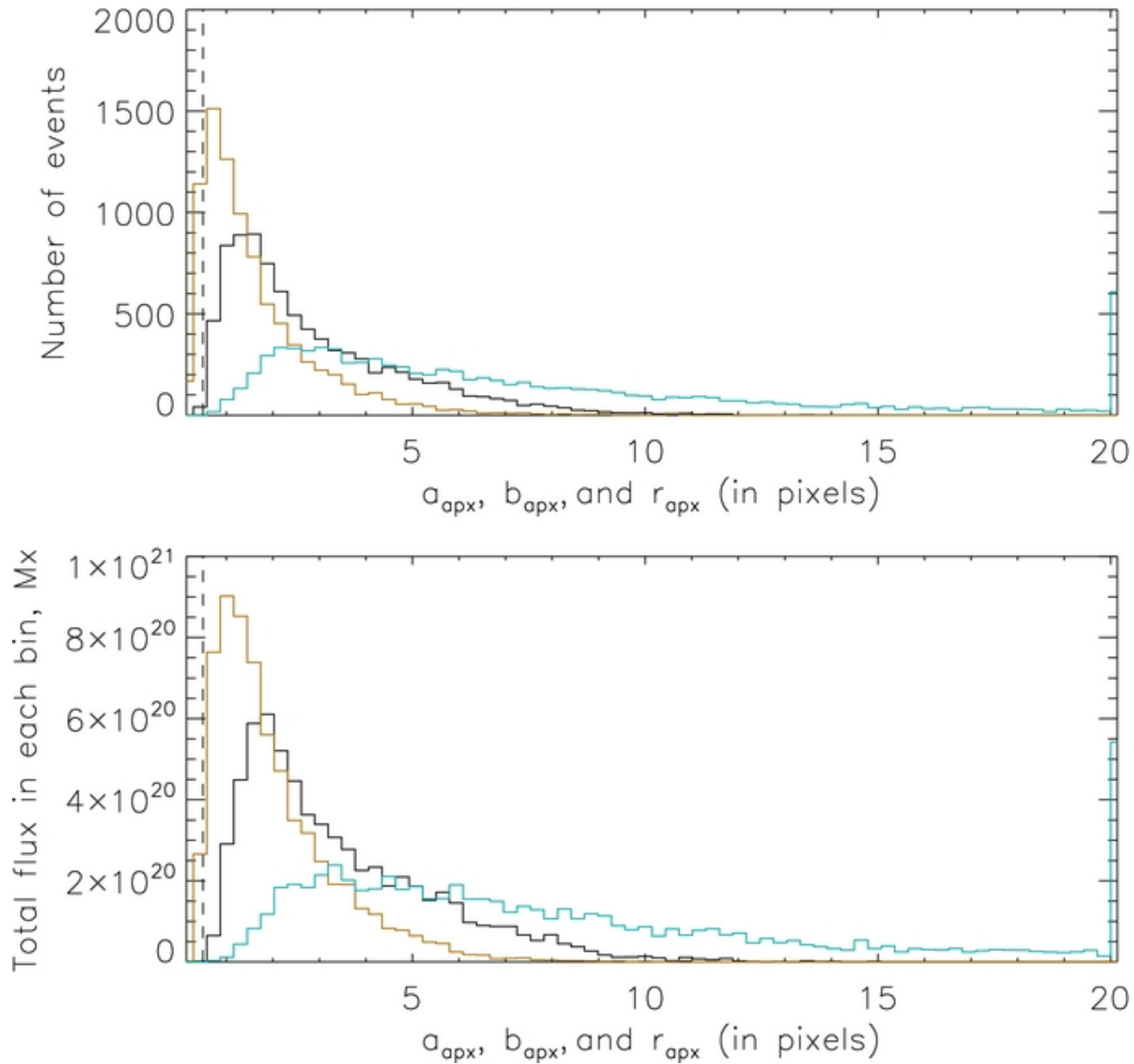
Figure 8. from On the Anisotropy in Expansion of Magnetic Flux Tubes in the Solar Corona Malanushenko & Schrijver 2013 ApJ 775 120 doi:10.1088/0004-637X/775/2/120 https://dx.doi.org/10.1088/0004-637X/775/2/120
