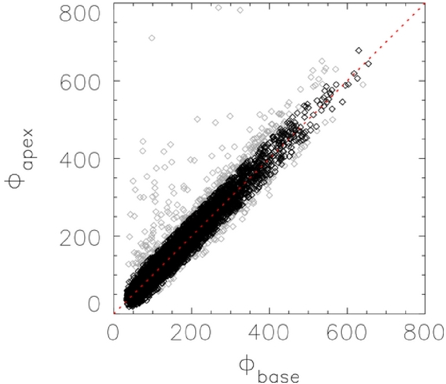
Figure 7. from On the Anisotropy in Expansion of Magnetic Flux Tubes in the Solar Corona Malanushenko & Schrijver 2013 ApJ 775 120 doi:10.1088/0004-637X/775/2/120 https://dx.doi.org/10.1088/0004-637X/775/2/120 © 2013. The American Astronomical Society. All rights reserved.
