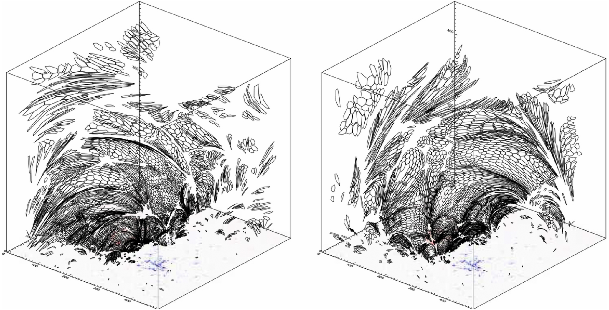
Figure 6. from On the Anisotropy in Expansion of Magnetic Flux Tubes in the Solar Corona Malanushenko & Schrijver 2013 ApJ 775 120 doi:10.1088/0004-637X/775/2/120 https://dx.doi.org/10.1088/0004-637X/775/2/120 © 2013. The American Astronomical Society. All rights reserved.
