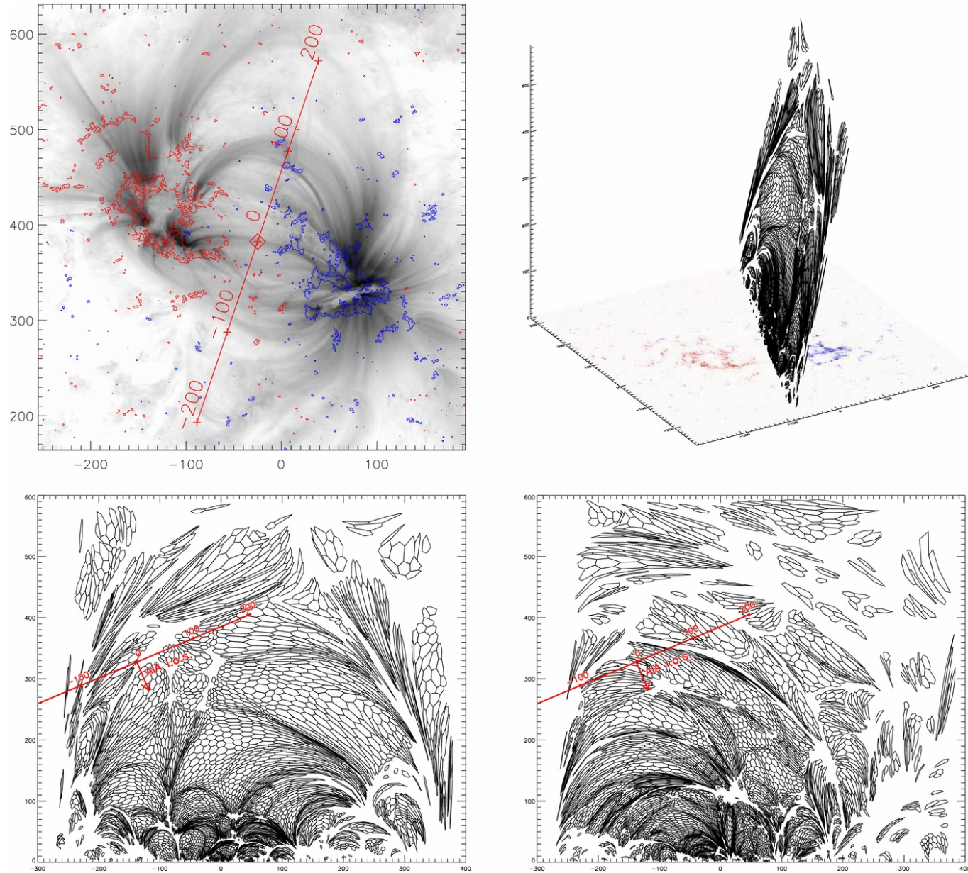
Figure 5. from On the Anisotropy in Expansion of Magnetic Flux Tubes in the Solar Corona Malanushenko & Schrijver 2013 ApJ 775 120 doi:10.1088/0004-637X/775/2/120 https://dx.doi.org/10.1088/0004-637X/775/2/120 © 2013. The American Astronomical Society. All rights reserved.
