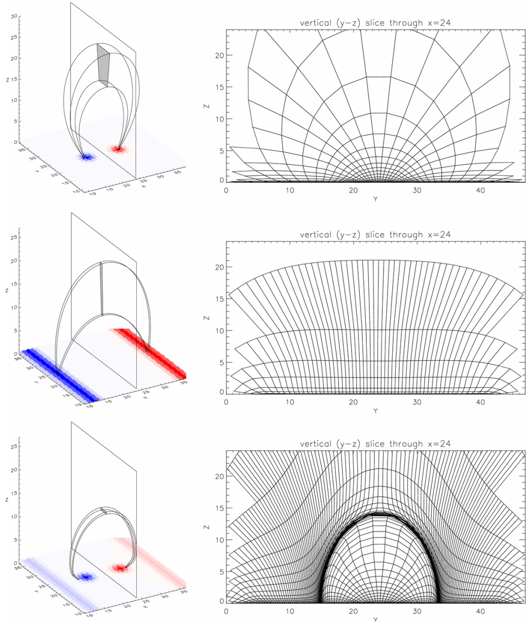
Figure 4. from On the Anisotropy in Expansion of Magnetic Flux Tubes in the Solar Corona Malanushenko & Schrijver 2013 ApJ 775 120 doi:10.1088/0004-637X/775/2/120 https://dx.doi.org/10.1088/0004-637X/775/2/120 © 2013. The American Astronomical Society. All rights reserved.
