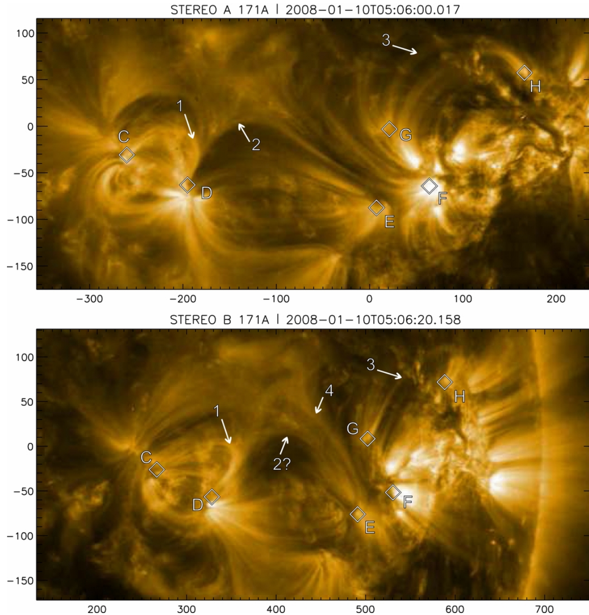
Figure 3. from On the Anisotropy in Expansion of Magnetic Flux Tubes in the Solar Corona Malanushenko & Schrijver 2013 ApJ 775 120 doi:10.1088/0004-637X/775/2/120 https://dx.doi.org/10.1088/0004-637X/775/2/120
