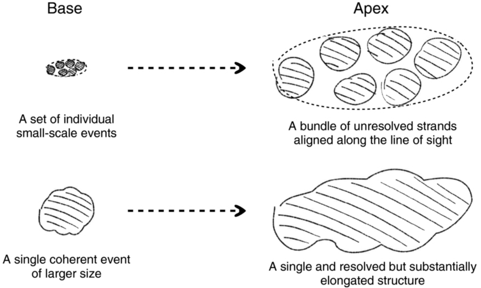
Figure 21. from On the Anisotropy in Expansion of Magnetic Flux Tubes in the Solar Corona Malanushenko & Schrijver 2013 ApJ 775 120 doi:10.1088/0004-637X/775/2/120 https://dx.doi.org/10.1088/0004-637X/775/2/120 © 2013. The American Astronomical Society. All rights reserved.
