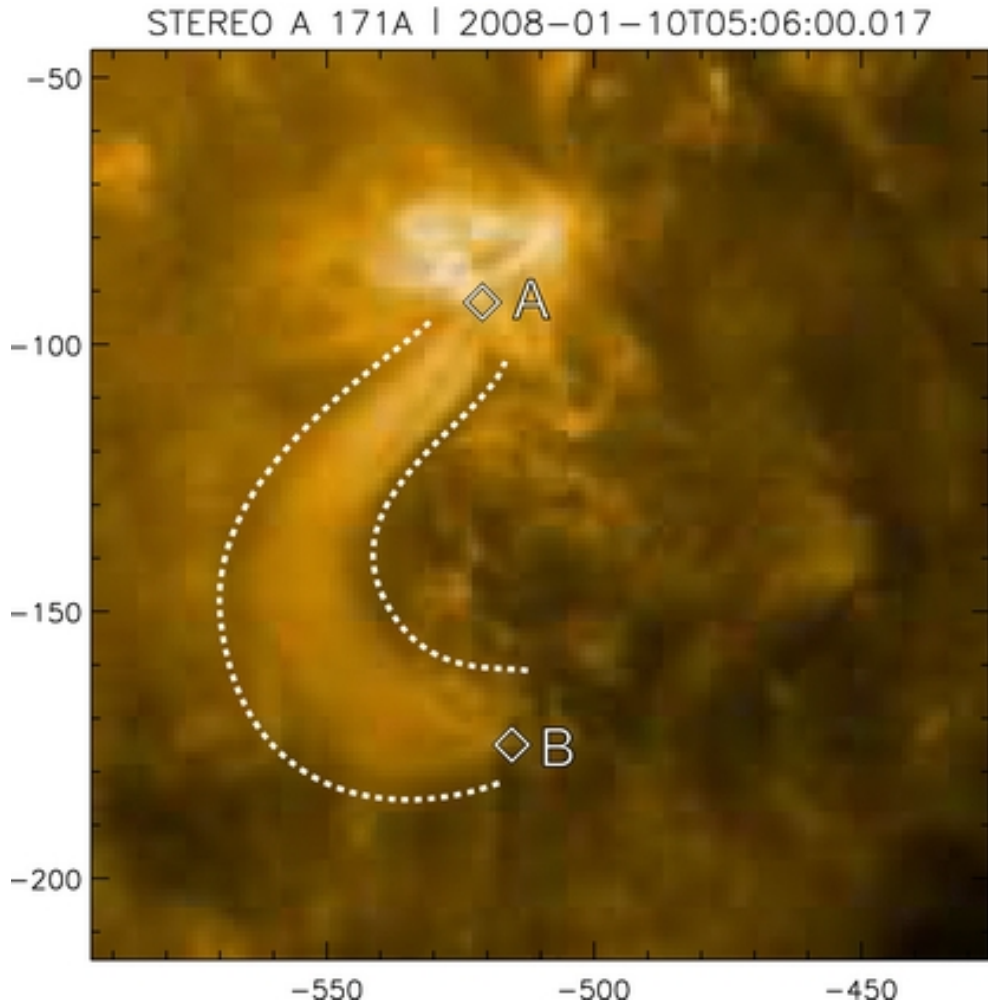
Figure 2. from On the Anisotropy in Expansion of Magnetic Flux Tubes in the Solar Corona Malanushenko & Schrijver 2013 ApJ 775 120 doi:10.1088/0004-637X/775/2/120 https://dx.doi.org/10.1088/0004-637X/775/2/120 © 2013. The American Astronomical Society. All rights reserved.
