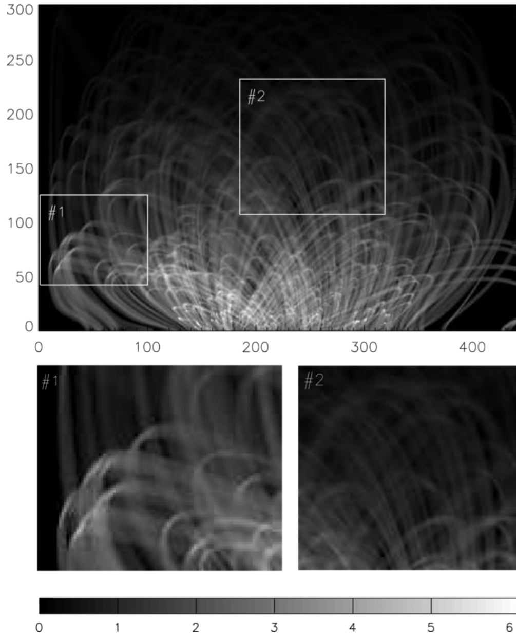
Figure 17. from On the Anisotropy in Expansion of Magnetic Flux Tubes in the Solar Corona Malanushenko & Schrijver 2013 ApJ 775 120 doi:10.1088/0004-637X/775/2/120 https://dx.doi.org/10.1088/0004-637X/775/2/120
