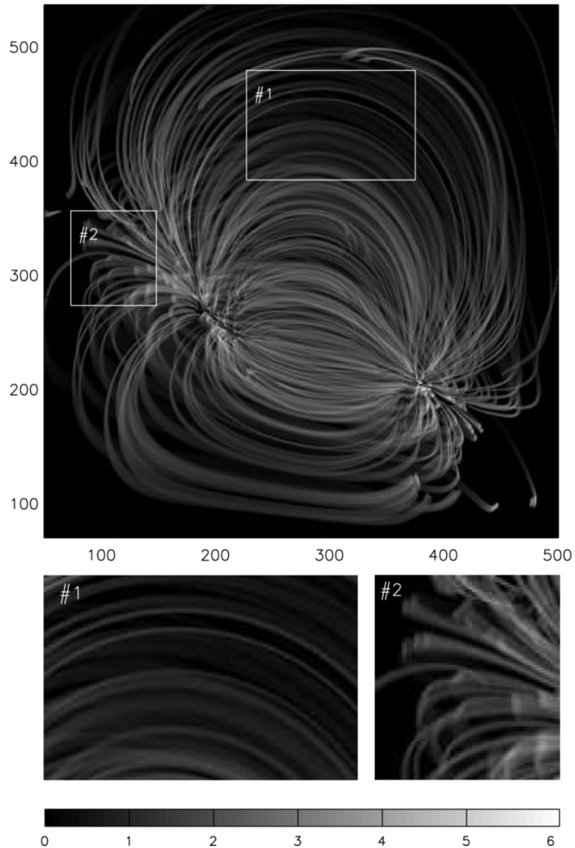
Figure 16. from On the Anisotropy in Expansion of Magnetic Flux Tubes in the Solar Corona Malanushenko & Schrijver 2013 ApJ 775 120 doi:10.1088/0004-637X/775/2/120 https://dx.doi.org/10.1088/0004-637X/775/2/120 © 2013. The American Astronomical Society. All rights reserved.
