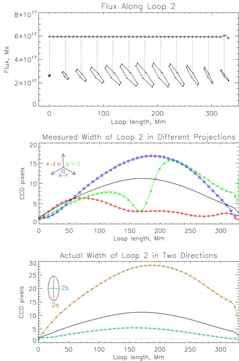
Figure 15. from On the Anisotropy in Expansion of Magnetic Flux Tubes in the Solar Corona Malanushenko & Schrijver 2013 ApJ 775 120 doi:10.1088/0004-637X/775/2/120 https://dx.doi.org/10.1088/0004-637X/775/2/120 © 2013. The American Astronomical Society. All rights reserved.
