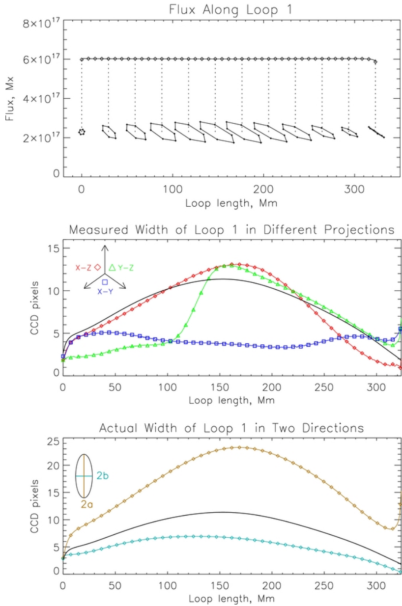
Figure 14. from On the Anisotropy in Expansion of Magnetic Flux Tubes in the Solar Corona Malanushenko & Schrijver 2013 ApJ 775 120 doi:10.1088/0004-637X/775/2/120 https://dx.doi.org/10.1088/0004-637X/775/2/120 © 2013. The American Astronomical Society. All rights reserved.
