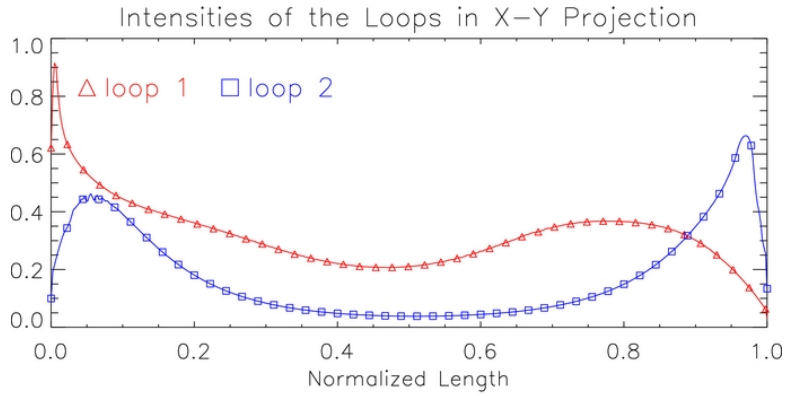
Figure 13. from On the Anisotropy in Expansion of Magnetic Flux Tubes in the Solar Corona Malanushenko & Schrijver 2013 ApJ 775 120 doi:10.1088/0004-637X/775/2/120 https://dx.doi.org/10.1088/0004-637X/775/2/120 © 2013. The American Astronomical Society. All rights reserved.
