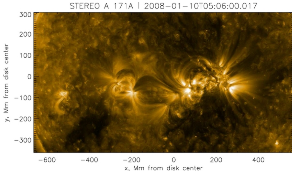
Figure 1. from On the Anisotropy in Expansion of Magnetic Flux Tubes in the Solar Corona Malanushenko & Schrijver 2013 ApJ 775 120 doi:10.1088/0004-637X/775/2/120 https://dx.doi.org/10.1088/0004-637X/775/2/120 © 2013. The American Astronomical Society. All rights reserved.
