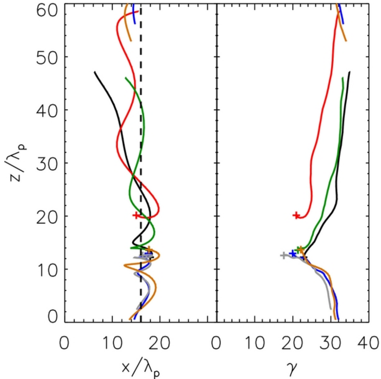
Figure 9. from A Flux Rope Network and Particle Acceleration in Three-dimensional Relativistic Magnetic Reconnection Kagan, Milosavljević, & Spitkovsky 2013 ApJ 774 41 doi:10.1088/0004-637X/774/1/41 https://dx.doi.org/10.1088/0004-637X/774/1/41 © 2013. The American Astronomical Society. All rights reserved.
