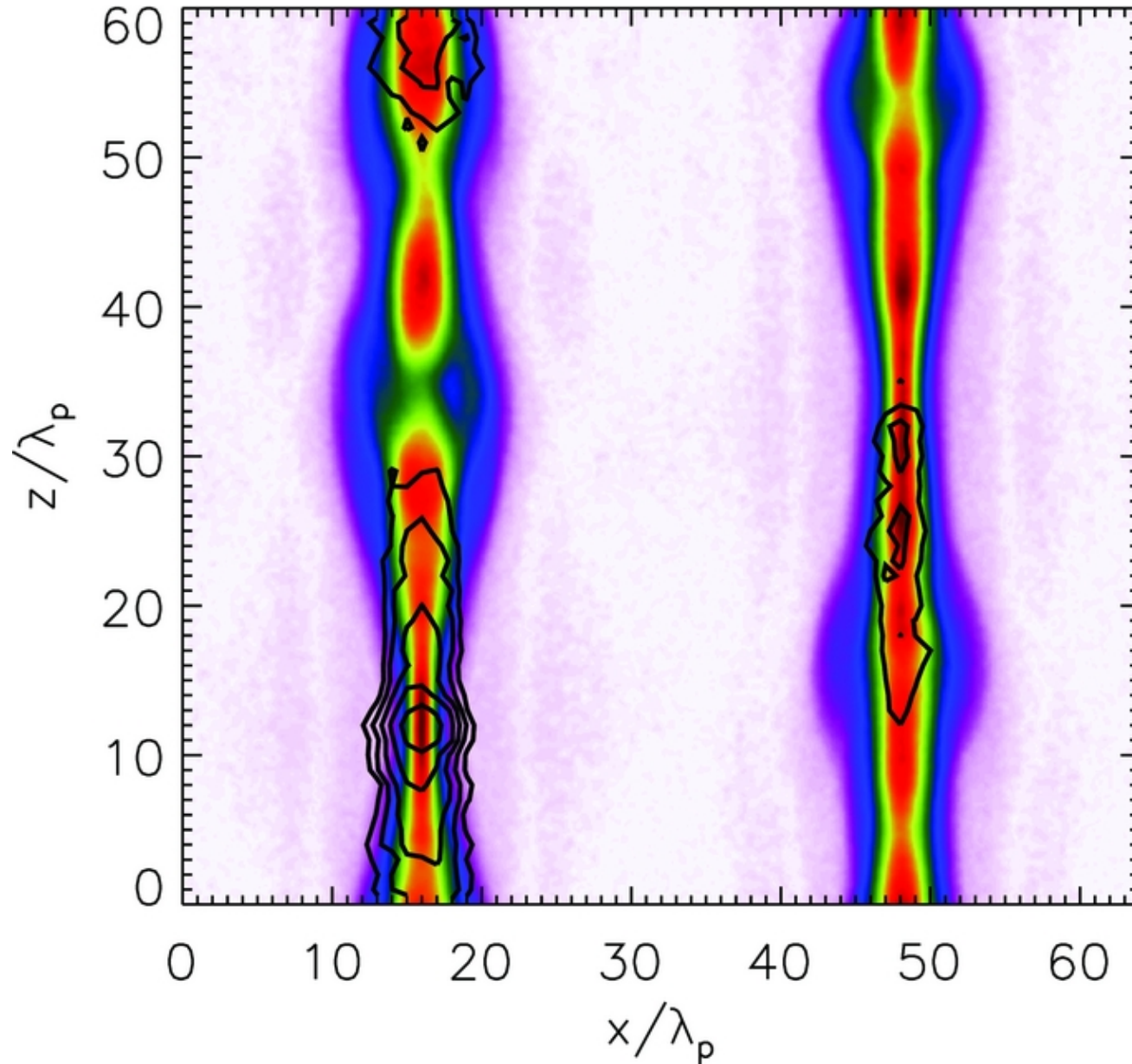
Figure 8. from A Flux Rope Network and Particle Acceleration in Three-dimensional Relativistic Magnetic Reconnection Kagan, Milosavljević, & Spitkovsky 2013 ApJ 774 41 doi:10.1088/0004-637X/774/1/41 https://dx.doi.org/10.1088/0004-637X/774/1/41 © 2013. The American Astronomical Society. All rights reserved.
