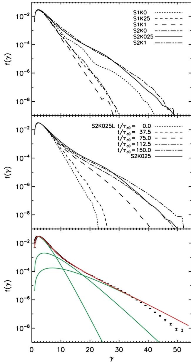
Figure 7. from A Flux Rope Network and Particle Acceleration in Three-dimensional Relativistic Magnetic Reconnection Kagan, Milosavljević, & Spitkovsky 2013 ApJ 774 41 doi:10.1088/0004-637X/774/1/41 https://dx.doi.org/10.1088/0004-637X/774/1/41
