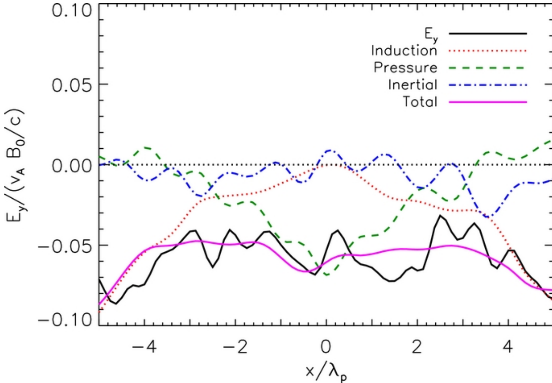
Figure 5. from A Flux Rope Network and Particle Acceleration in Three-dimensional Relativistic Magnetic Reconnection Kagan, Milosavljević, & Spitkovsky 2013 ApJ 774 41 doi:10.1088/0004-637X/774/1/41 https://dx.doi.org/10.1088/0004-637X/774/1/41
