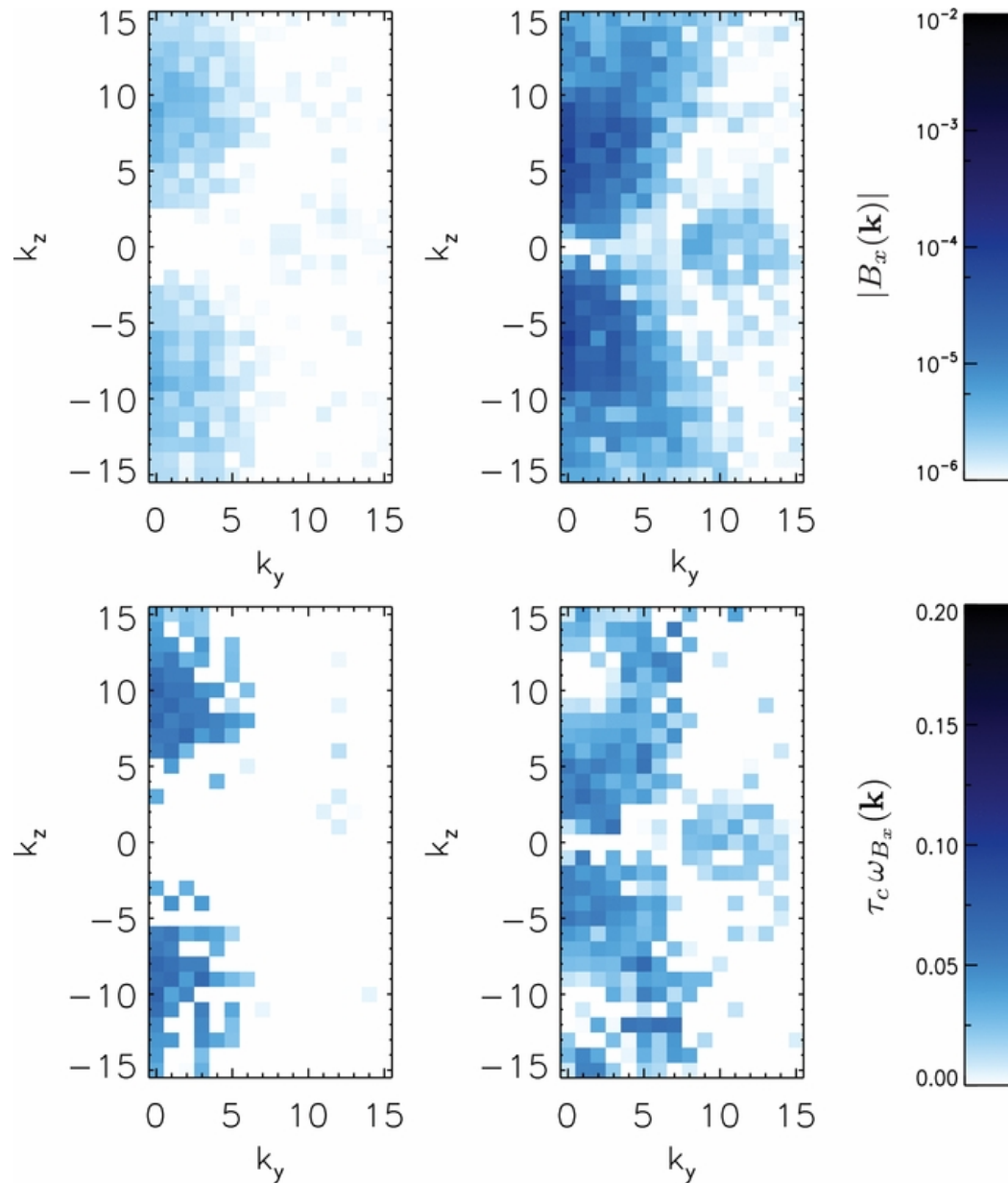
Figure 4. from A Flux Rope Network and Particle Acceleration in Three-dimensional Relativistic Magnetic Reconnection Kagan, Milosavljević, & Spitkovsky 2013 ApJ 774 41 doi:10.1088/0004-637X/774/1/41 https://dx.doi.org/10.1088/0004-637X/774/1/41
