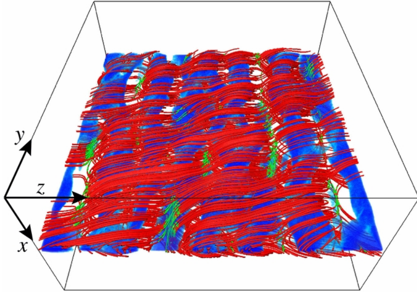
Figure 3. from A Flux Rope Network and Particle Acceleration in Three-dimensional Relativistic Magnetic Reconnection Kagan, Milosavljević, & Spitkovsky 2013 ApJ 774 41 doi:10.1088/0004-637X/774/1/41 https://dx.doi.org/10.1088/0004-637X/774/1/41 © 2013. The American Astronomical Society. All rights reserved.
