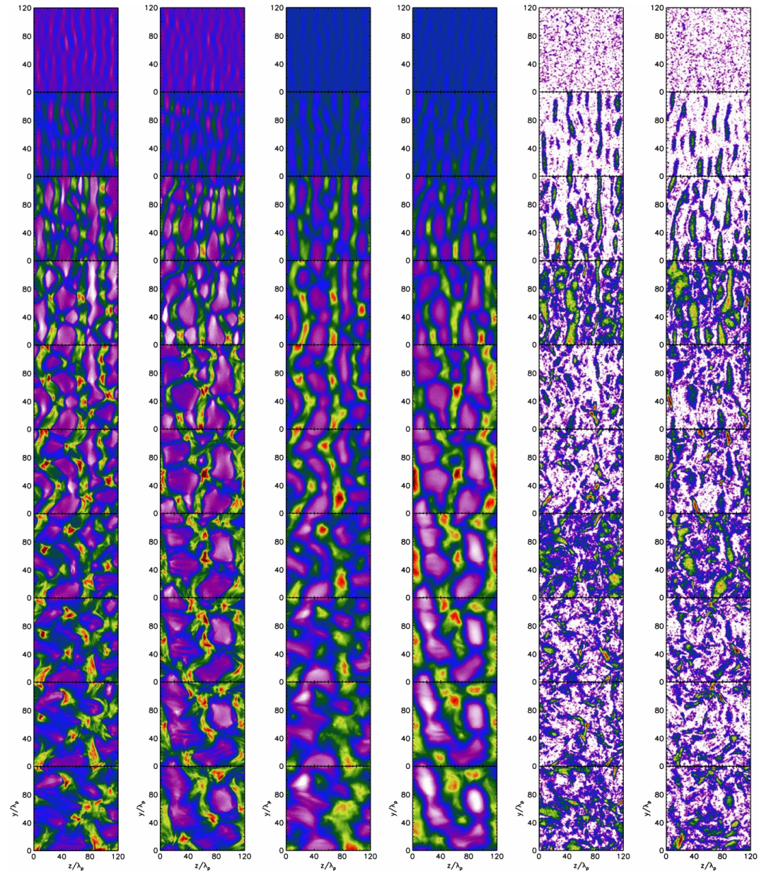
Figure 2. from A Flux Rope Network and Particle Acceleration in Three-dimensional Relativistic Magnetic Reconnection Kagan, Milosavljević, & Spitkovsky 2013 ApJ 774 41 doi:10.1088/0004-637X/774/1/41 https://dx.doi.org/10.1088/0004-637X/774/1/41
