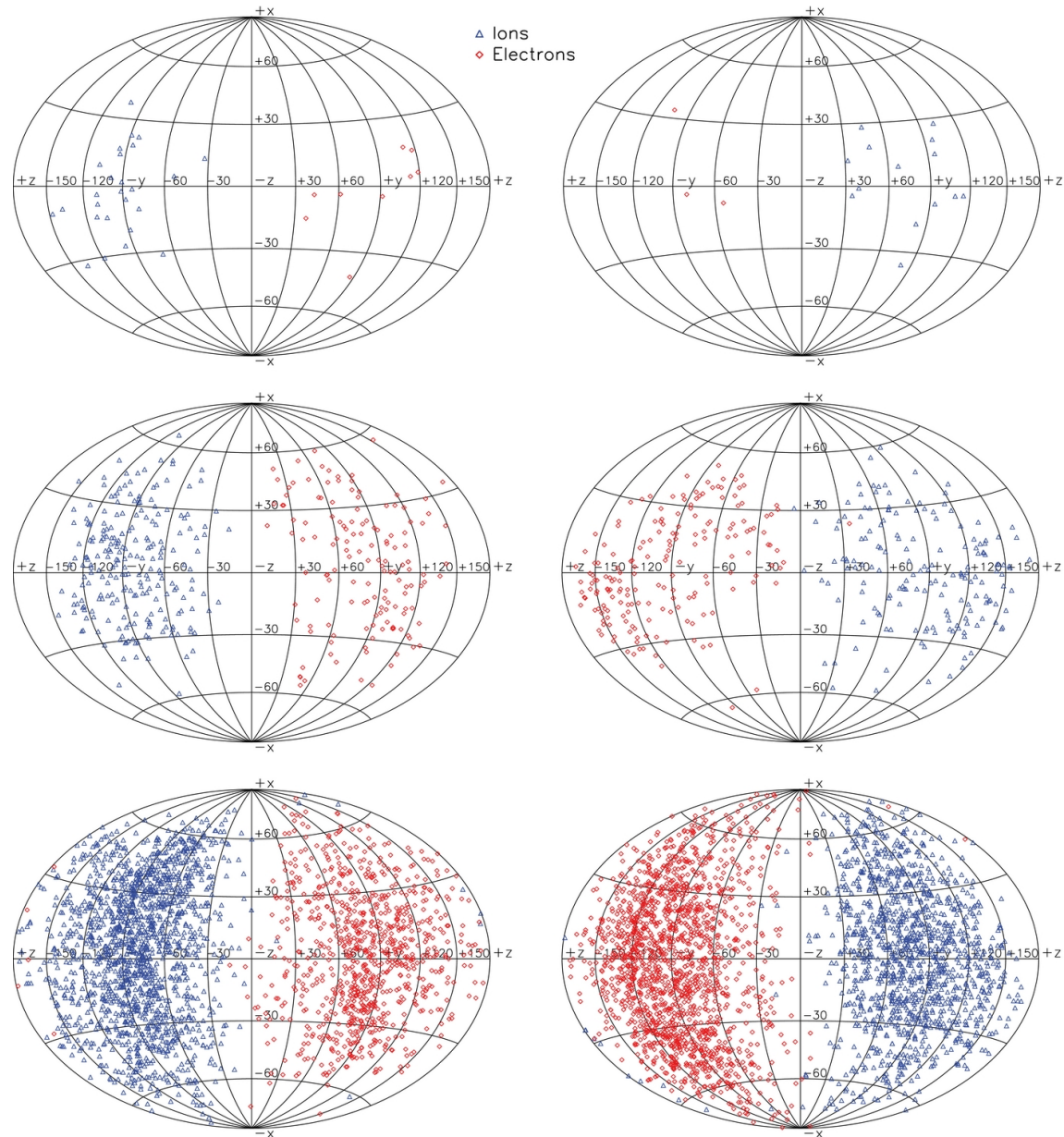
Figure 10. from A Flux Rope Network and Particle Acceleration in Three-dimensional Relativistic Magnetic Reconnection Kagan, Milosavljević, & Spitkovsky 2013 ApJ 774 41 doi:10.1088/0004-637X/774/1/41 https://dx.doi.org/10.1088/0004-637X/774/1/41
