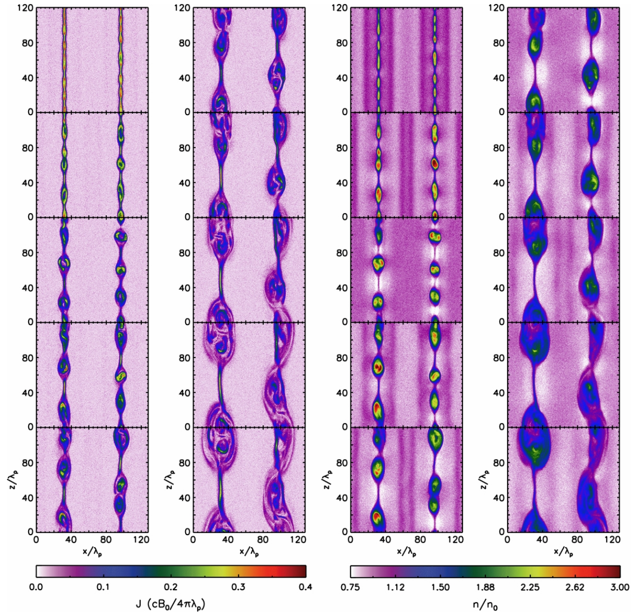
Figure 1. from A Flux Rope Network and Particle Acceleration in Three-dimensional Relativistic Magnetic Reconnection Kagan, Milosavljević, & Spitkovsky 2013 ApJ 774 41 doi:10.1088/0004-637X/774/1/41 https://dx.doi.org/10.1088/0004-637X/774/1/41
