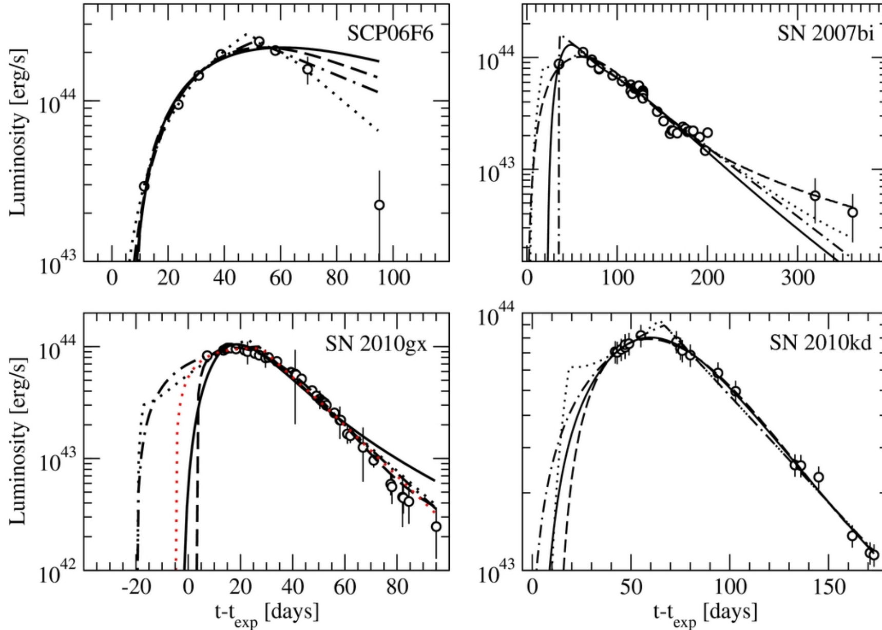
Figure 4. from Analytical Light Curve Models of Superluminous Supernovae: 2-minimization of Parameter Fits Chatzopoulos et al. 2013 ApJ 773 76 doi:10.1088/0004-637X/773/1/76 https://dx.doi.org/10.1088/0004-637X/773/1/76 © 2013. The American Astronomical Society. All rights reserved.
