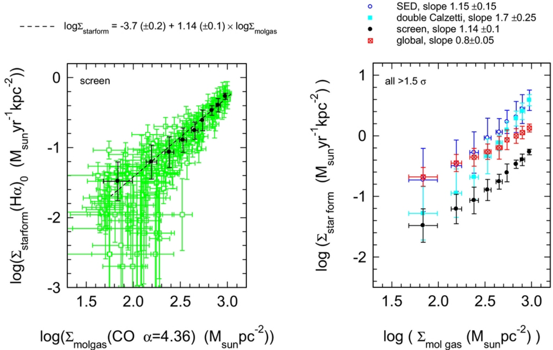
Figure 8. from Phibss: Molecular Gas, Extinction, Star Formation, and Kinematics in the z = 1.5 Star-forming Galaxy EGS13011166 Genzel et al. 2013 ApJ 773 68 doi:10.1088/0004-637X/773/1/68 https://dx.doi.org/10.1088/0004-637X/773/1/68 © 2013. The American Astronomical Society. All rights reserved.
