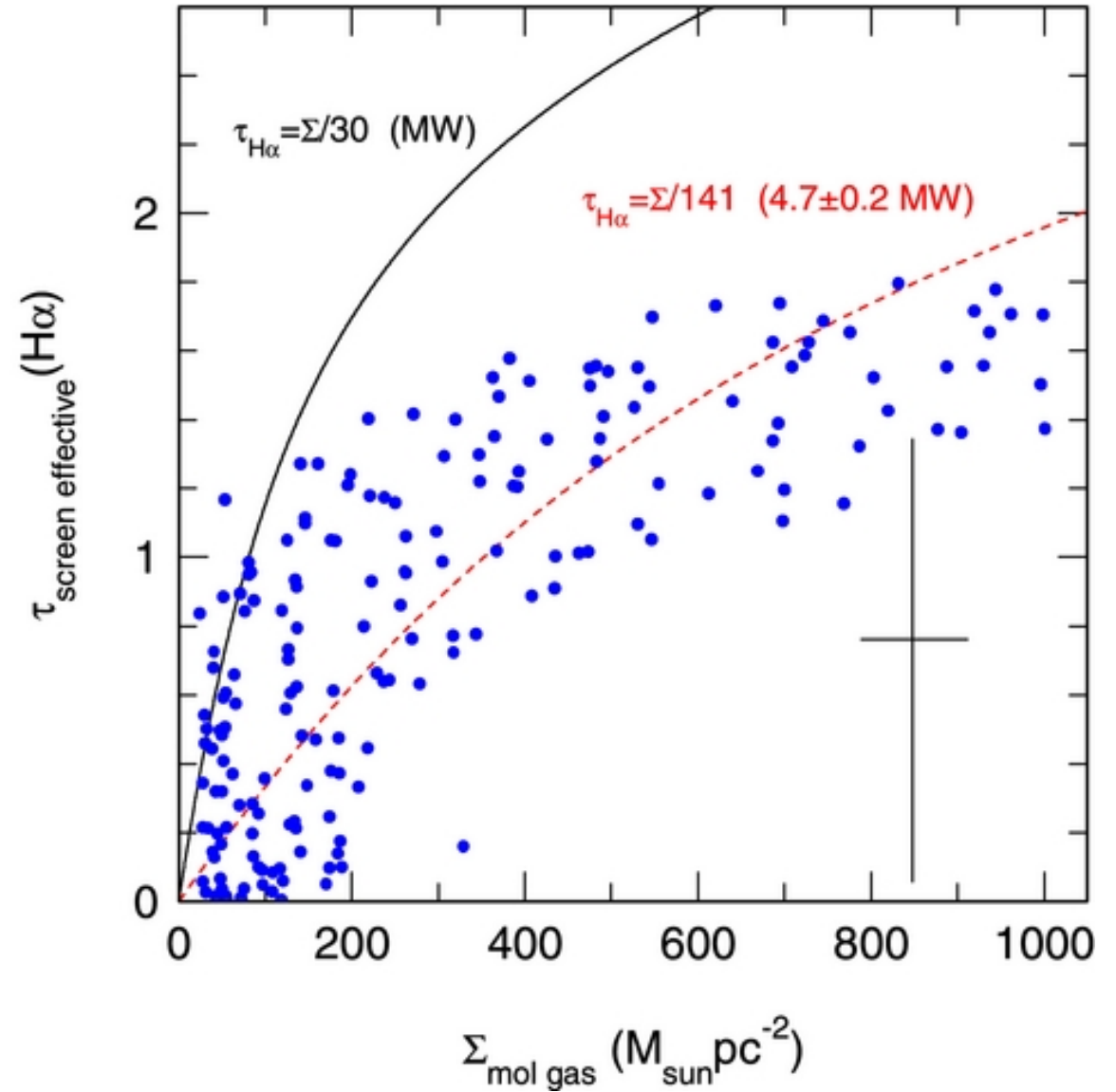
Figure 7. from Phibss: Molecular Gas, Extinction, Star Formation, and Kinematics in the z = 1.5 Star-forming Galaxy EGS13011166 Genzel et al. 2013 ApJ 773 68 doi:10.1088/0004-637X/773/1/68 https://dx.doi.org/10.1088/0004-637X/773/1/68 © 2013. The American Astronomical Society. All rights reserved.
