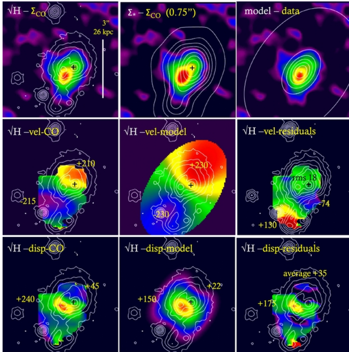
Figure 4. from Phibss: Molecular Gas, Extinction, Star Formation, and Kinematics in the z = 1.5 Star-forming Galaxy EGS13011166 Genzel et al. 2013 ApJ 773 68 doi:10.1088/0004-637X/773/1/68 https://dx.doi.org/10.1088/0004-637X/773/1/68 © 2013. The American Astronomical Society. All rights reserved.
