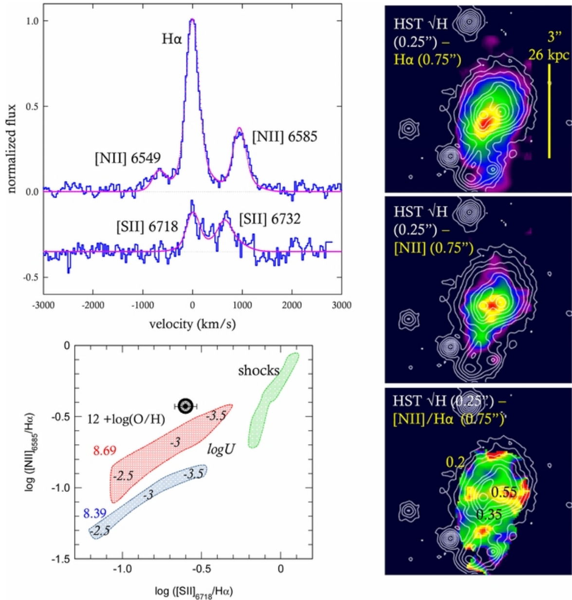
Figure 3. from Phibbs: Molecular Gas, Extinction, Star Formation, and Kinematics in the z = 1.5 Star-forming Galaxy EGS13011166 Genzel et al. 2013 ApJ 773 68 doi:10.1088/0004-637X/773/1/68 https://dx.doi.org/10.1088/0004-637X/773/1/68 © 2013. The American Astronomical Society. All rights reserved.
