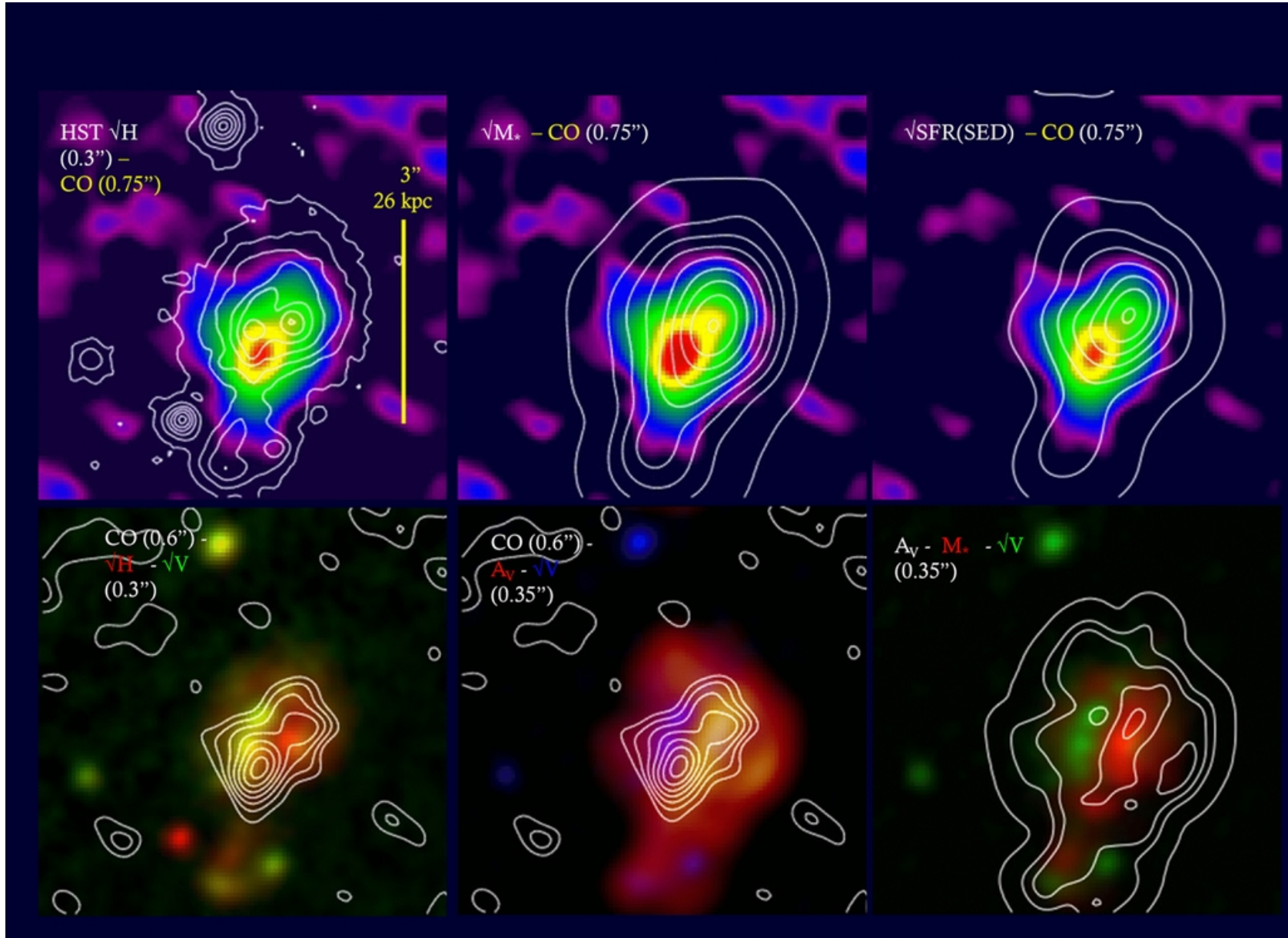
Figure 2. from Phibss: Molecular Gas, Extinction, Star Formation, and Kinematics in the z = 1.5 Star-forming Galaxy EGS13011166 Genzel et al. 2013 ApJ 773 68 doi:10.1088/0004-637X/773/1/68 https://dx.doi.org/10.1088/0004-637X/773/1/68 © 2013. The American Astronomical Society. All rights reserved.
