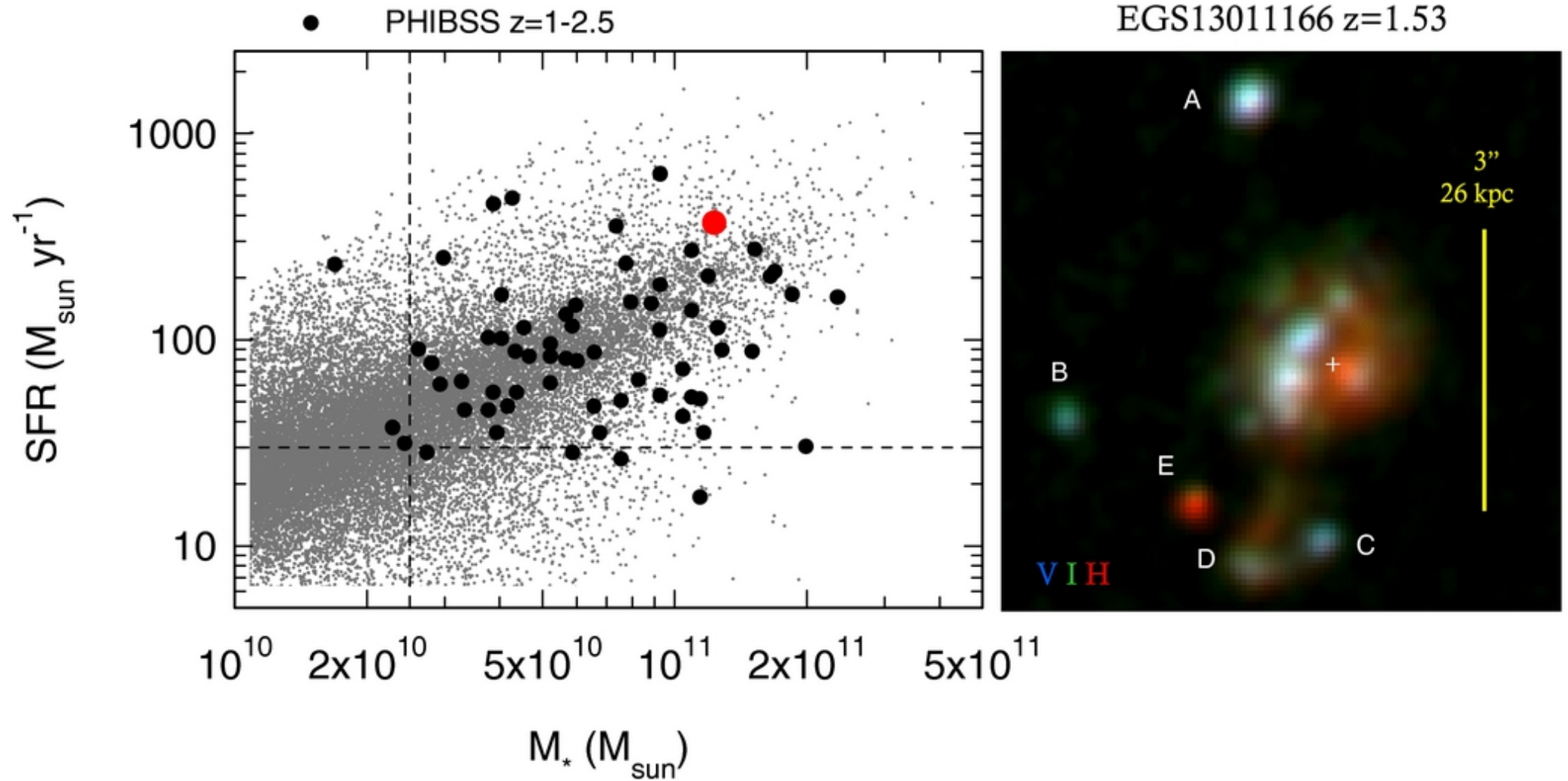
Figure 1. from Phibss: Molecular Gas, Extinction, Star Formation, and Kinematics in the z = 1.5 Star-forming Galaxy EGS13011166 Genzel et al. 2013 ApJ 773 68 doi:10.1088/0004-637X/773/1/68 https://dx.doi.org/10.1088/0004-637X/773/1/68 © 2013. The American Astronomical Society. All rights reserved.
