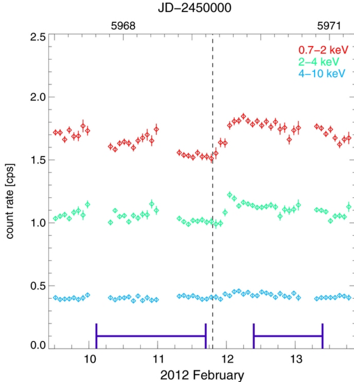
Figure 7. from An X-Ray View of the Jet Cycle in the Radio-loud AGN 3C120 Lohfink et al. 2013 ApJ 772 83 doi:10.1088/0004-637X/772/2/83 https://dx.doi.org/10.1088/0004-637X/772/2/83 © 2013. The American Astronomical Society. All rights reserved.
