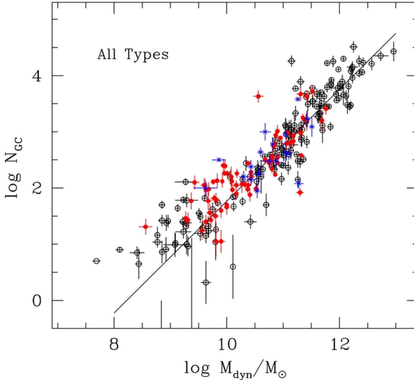
Figure 9. from A Catalog of Globular Cluster Systems: What Determines the Size of a Galaxy's Globular Cluster Population? Harris, Harris, & Alessi 2013 ApJ 772 82 doi:10.1088/0004-637X/772/2/82 https://dx.doi.org/10.1088/0004-637X/772/2/82 © 2013. The American Astronomical Society. All rights reserved.
